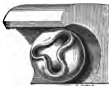
134. The ball-flower.
